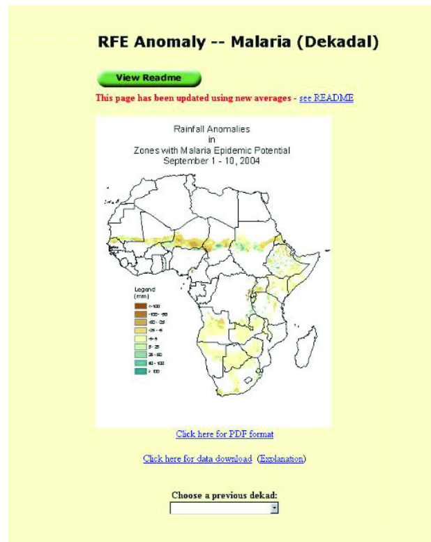
Fig. 4. Rain Fall Anomaly (for Malaria) produced every decade with a spatial resolution of 10 km. Data are available on the website of the USGS, Africa Data Dissemination Service: http://igskmnchwb015.cr.usgs.gov/adds/ .
